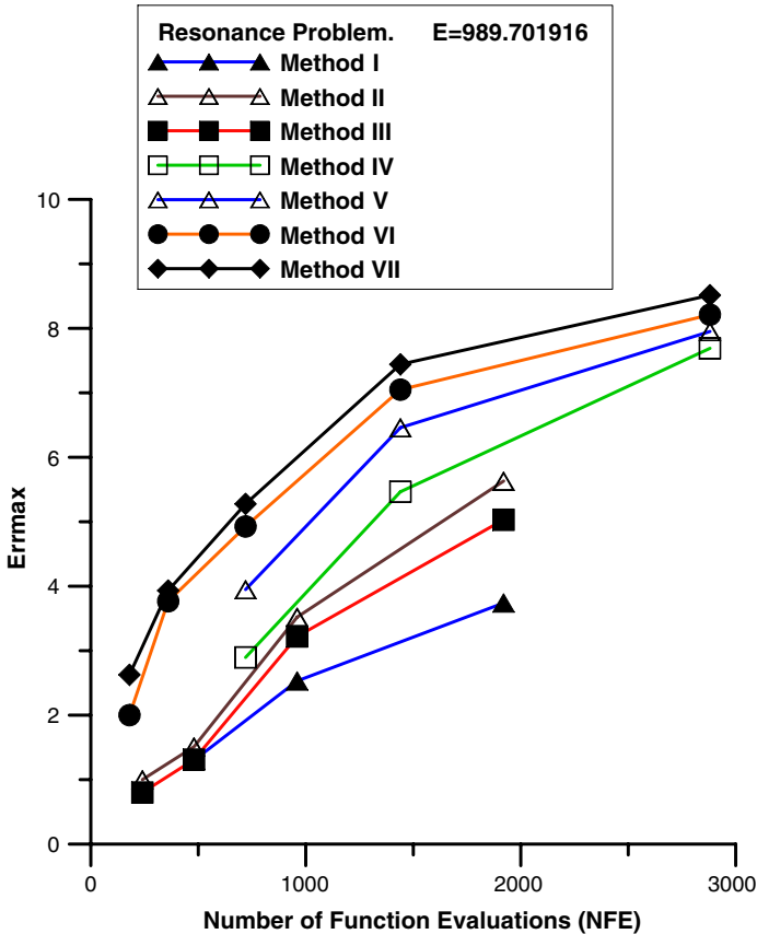
Fig. 12 Error Ermax for several values of n for the eigenvalue E_3 = 989.701916 . The nonexistence of a value of Ermax indicates that for this value of n , Ermax is positive
