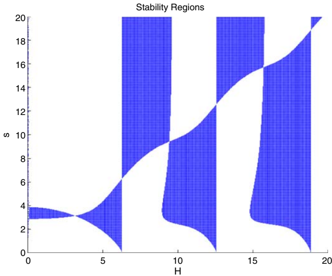
Fig. 5 s - H plane of the first method of the new family of method developed in this paper (paragraph 3.1)
