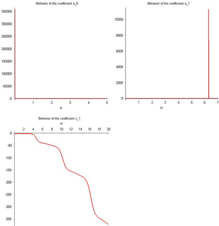
Fig. 2 Behavior of the coefficients of the new method given by (18) for several values of H
