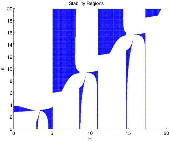
Fig. 8 s - H plane of the fourth method of the new family of method developed in this paper (paragraph 3.4)
