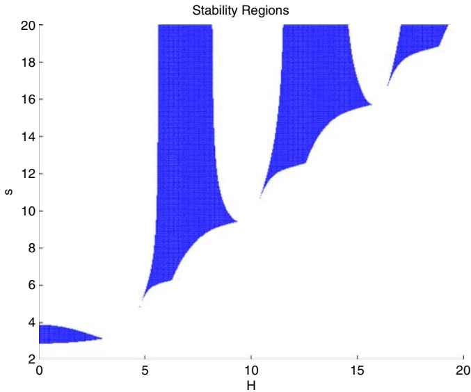
Fig. 6 s-H plane of the second method of the new family of method developed in this paper (paragraph 3.2)
