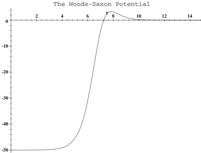
Fig. 10 The Woods-Saxon potential
