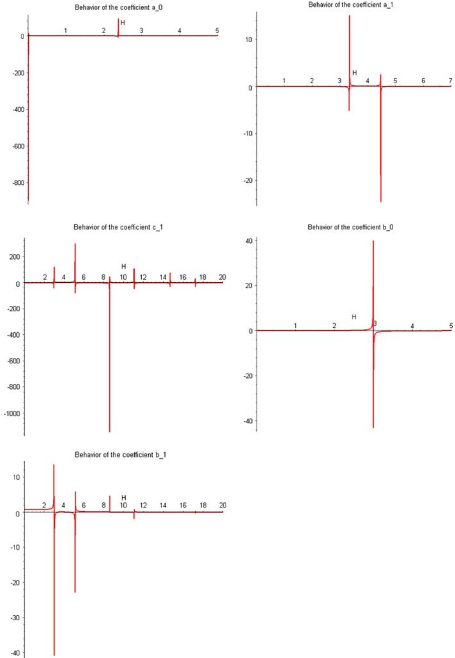
Fig. 4 Behavior of the coefficients of the new method given by (28) for several values of H
