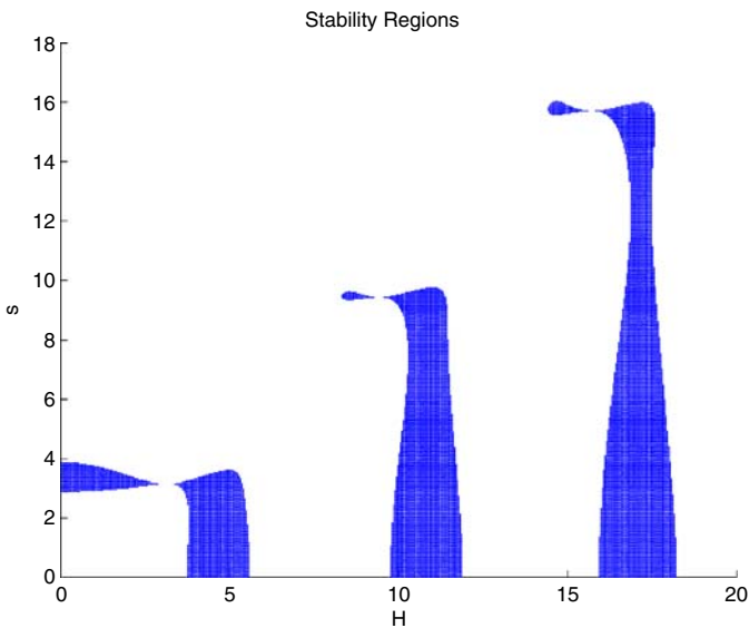
Fig. 7 s-H plane of the third method of the new family of method developed in this paper (paragraph 3.3)
