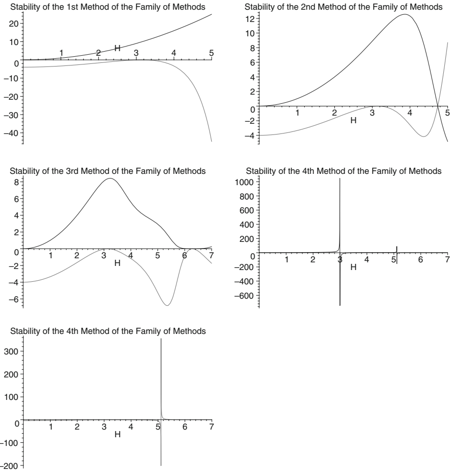
Fig. 9 Stability polynomials of the new developed methods in the case that H = s
