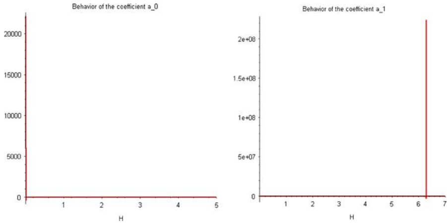
Fig. 1 Behavior of the coefficients of the new method given by (13) for several values of H
